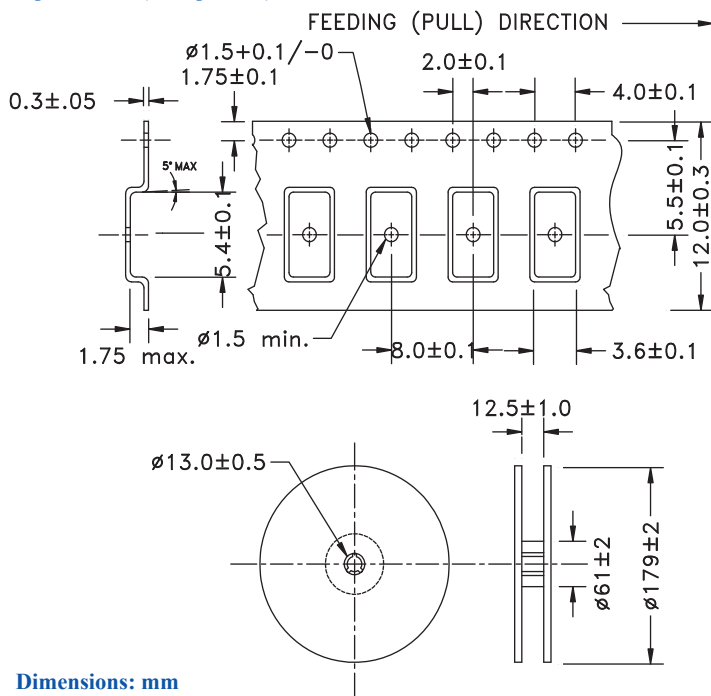
Tape and reel (1,000pcs/reel)
